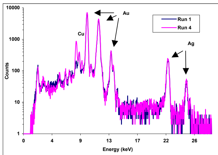
Figure 3. Comparison of #1 and #4. The difference in concentration of the copper peak at 8 keV indicates that the artists used more copper at the welds.
