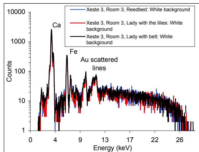
Figure 5. Comparison of three spectra taken from the white background of various wall paintings.
