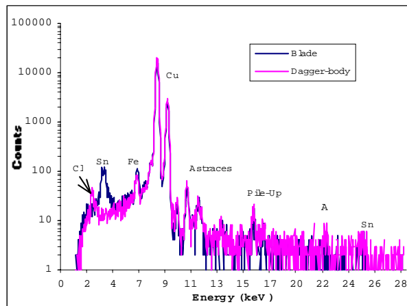
Figure 4. Comparison of the dagger (Mus. No. 8597) and blade (Mus. No. 6219) spectra.
